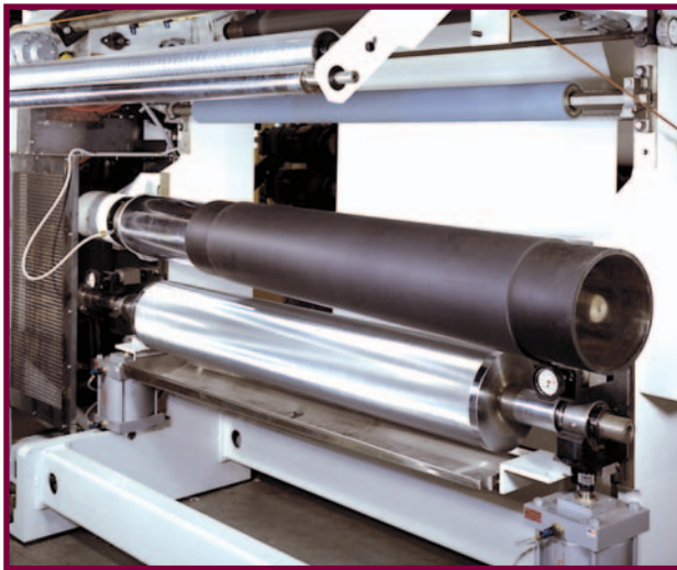
Gravure coater with "speed sleeve".
