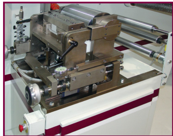
Slot/die coating module
