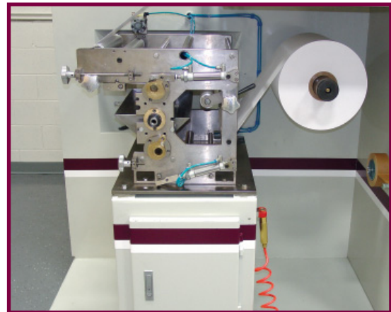
Roll coater module and unwind
